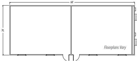
24' x 60' Classroom*
