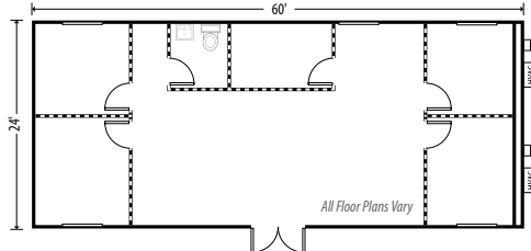
24' x 60' Sales Office*
